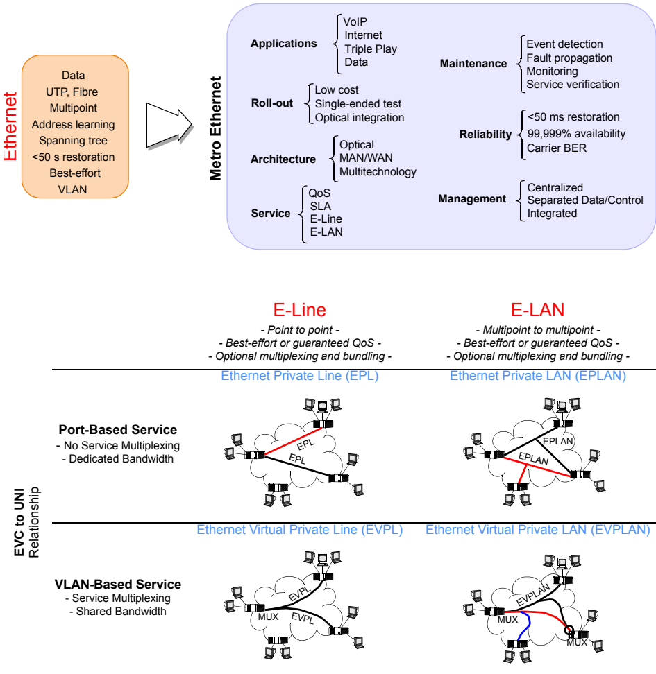
Figure 1 Generic Ethernet Service Type (Metro Ethernet Forum)
